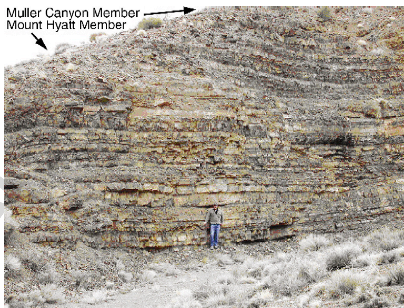
Fig. 3. Mount Hyatt Member (Rhaetian) in Muller Canyon area. The base of the overlying Muller Canyon Member is seen in the upper right side of the photograph. The lowest samples for isotope analysis in this study came from the base of this cliff.
