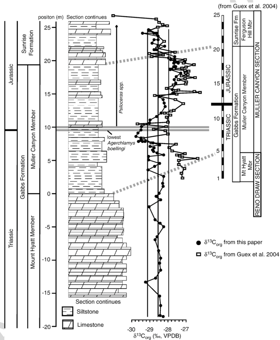
Fig. 6. The stratigraphic section and \delta^{13}C_{org} data measured by Guex et al. (2004) overlain on the section and \delta^{13}C_{org} from this paper. The two sections are aligned such that the structures of the \delta^{13}C_{org} curves match. Note that all the \delta^{13}C_{org} data presented in this paper were measured from samples collected from the same section (i.e. the Muller Canyon section), while the Guex et al. data are from two sections: Muller Canyon Member and Ferguson Hill Member samples were collected from the Muller Canyon section, and Mount Hyatt Member samples were collected from the Reno Draw section. The Reno Draw and Muller Canyon sections sit in structurally different blocks (Taylor et al., 1983). The differences in the two \delta^{13}C_{org} curves may be a result of incomplete de-carbonation (and thus the presence of recalcitrant, isotopically heavy material such as siderite) on the part of Guex et al. Furthermore, Guex et al. (2004) appear to have missed the lowermost ~8 m of the Muller Canyon Member at the Muller Canyon section. These units are not strongly competent, and the boundaries between units are somewhat indistinct.
