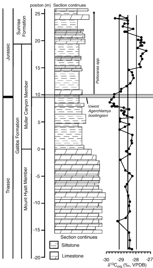
Fig. 5. Measured section at Ferguson Hill, Muller Canyon showing our litho-, bio-, and chemostratigraphic results. Width of lithological units relates to degree of induration as seen in field. Grey line marks base of Jurassic as picked by ammonites, whereas the first appearance of A. boellingi is favored here for the base of the Jurassic.
