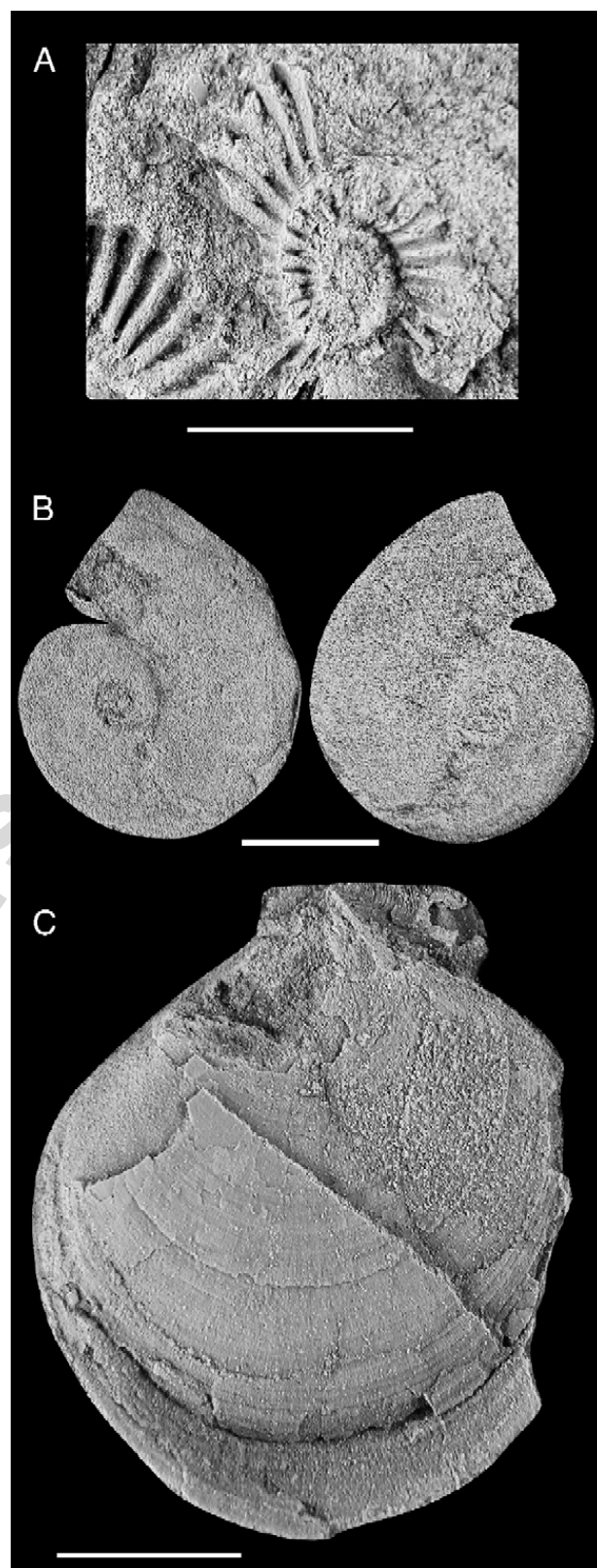
Fig. 4. Photographs of important index fossils and stratigraphic height of discovery above the Mount Hyatt–Muller Canyon boundary from Ferguson Hill, Nevada, USA. A. Possible Choristoceras crickmayi , 1 m; B. Psiloceras sp. 10.5 m; C. Agerchlamys boellingi , 9.6 m.
