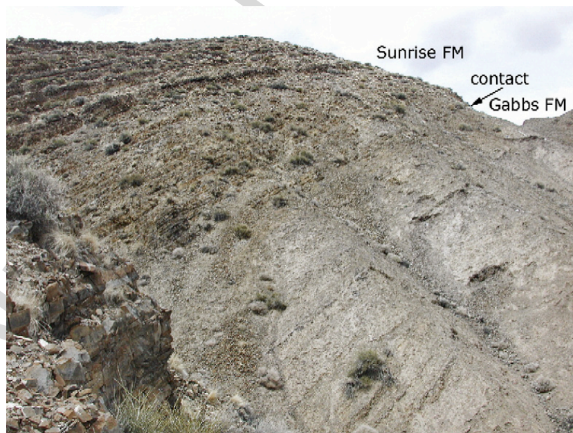
Fig. 1. View of Muller Canyon region showing the Muller Canyon Member of the Gabbs Formation (below) and Sunrise Formation (above). Black line marks contact between the units. The samples used in this study came from the small gully running nearly perpendicular to bedding from the lower right corner of the photograph. The Mount Hyatt Member of the Gabbs Formation is not visible in this photo, but is just beneath the lower right corner.
